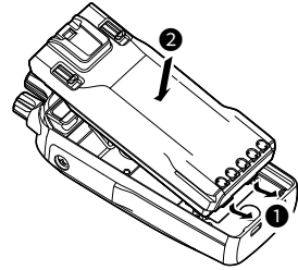
Battery sliding locks
