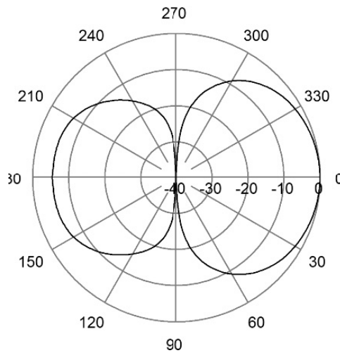
E-Plane | 98 MHz
