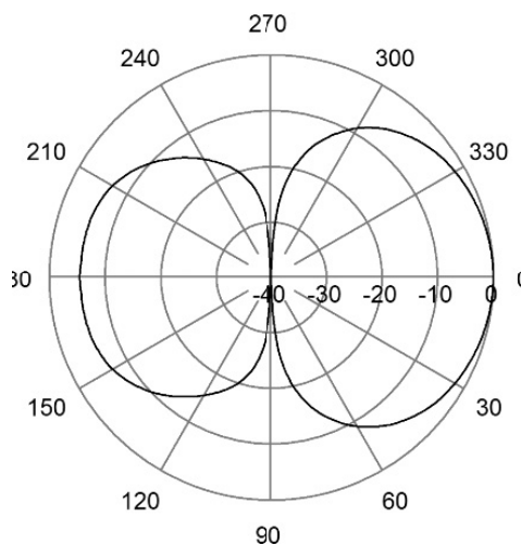
E-Plane | 459 MHz
