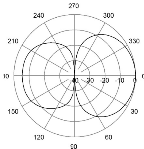
E-Plane | 405 MHz
