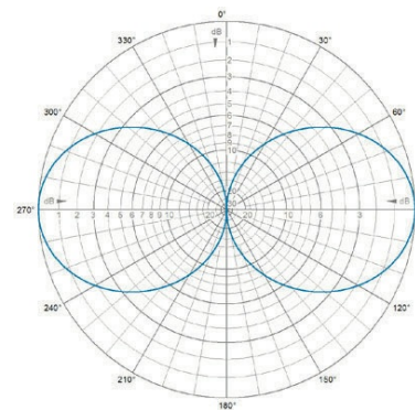
E-Plane | 132 MHz
